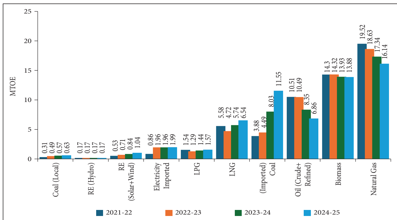
Figure 1: Primary Energy Supply Mix of Bangladesh
