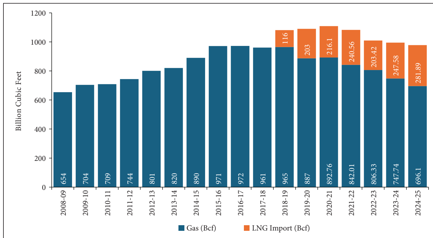
Figure 5: Historical Trend in Production of Gas (2009-2025) in Bcf
